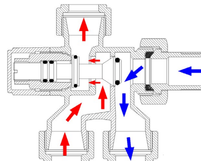
Fig. 1: fully open valve section (max flow rate to the radiator and minimum by-pass flow)
