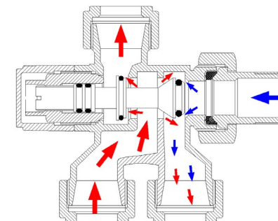
Fig. 2: single-pipe valve section (a certain quantity of fluid is supplied to the radiator and the remainder to the by-pass)
